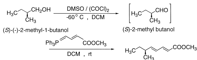
Figure 7. Synthesis of methyl (2E,4E,6S)-6-methyl-2,4-octadienoate.
