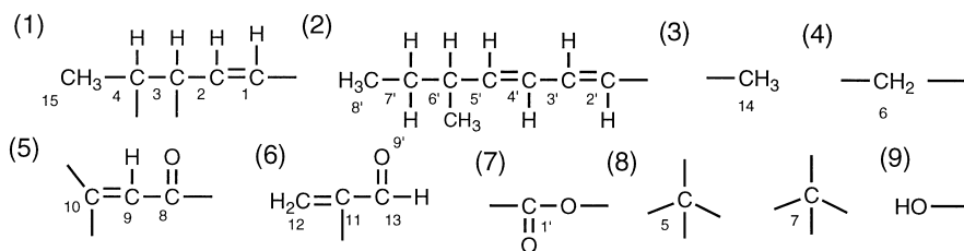
Figure 2. The partial structures of KM-01 (— implies quaternary carbons).
