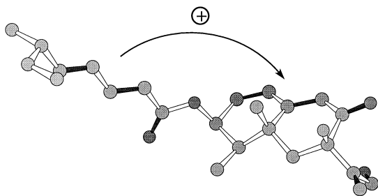
Figure 5. The most stable conformer of KM-01 calculated by the AMBER* force field.
