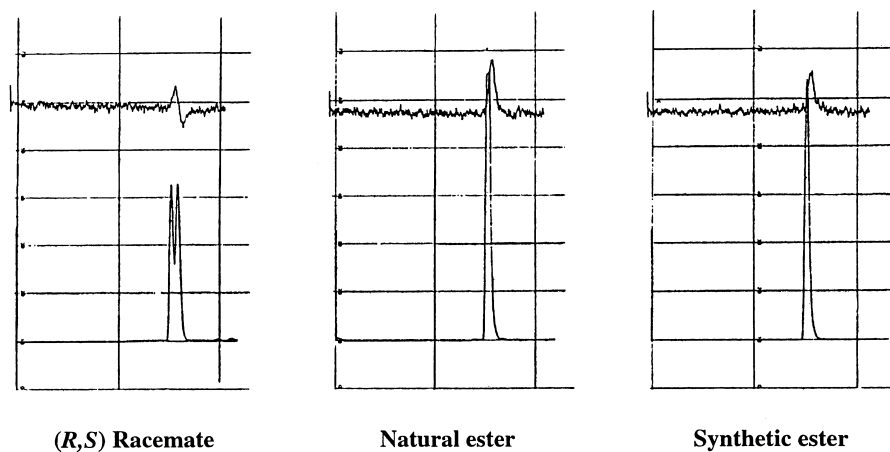
Figure 8. HPLC Chromatogram and polarimetric diagram for the resolution of racemate, natural and synthetic ester on a CHIR-ALCEL OD column.
