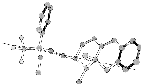
Figure 6. The lowest energy conformer of an analogue of ( S )-MTPA ester 4b . The dotted line indicates the MTPA plane. The quinoxaline moiety of the ( S )-MTPA-ester 4b is replaced by benzene in the analogue.
