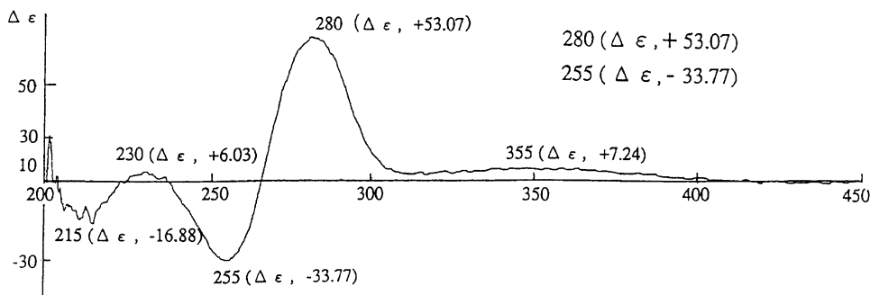
Figure 4. Splitting CD spectrum of KM-01.
