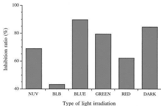
Figure 1. Production of KM-01 under various light irradiation.
