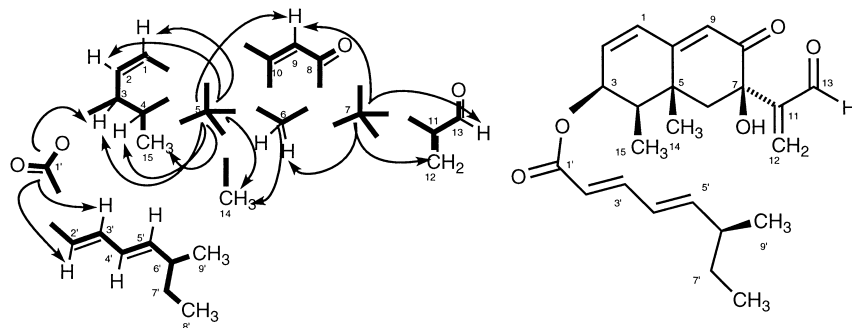
Figure 3. Carbon-proton connectivity by HMBC analysis (left) and the structures of KM-01 (right).
